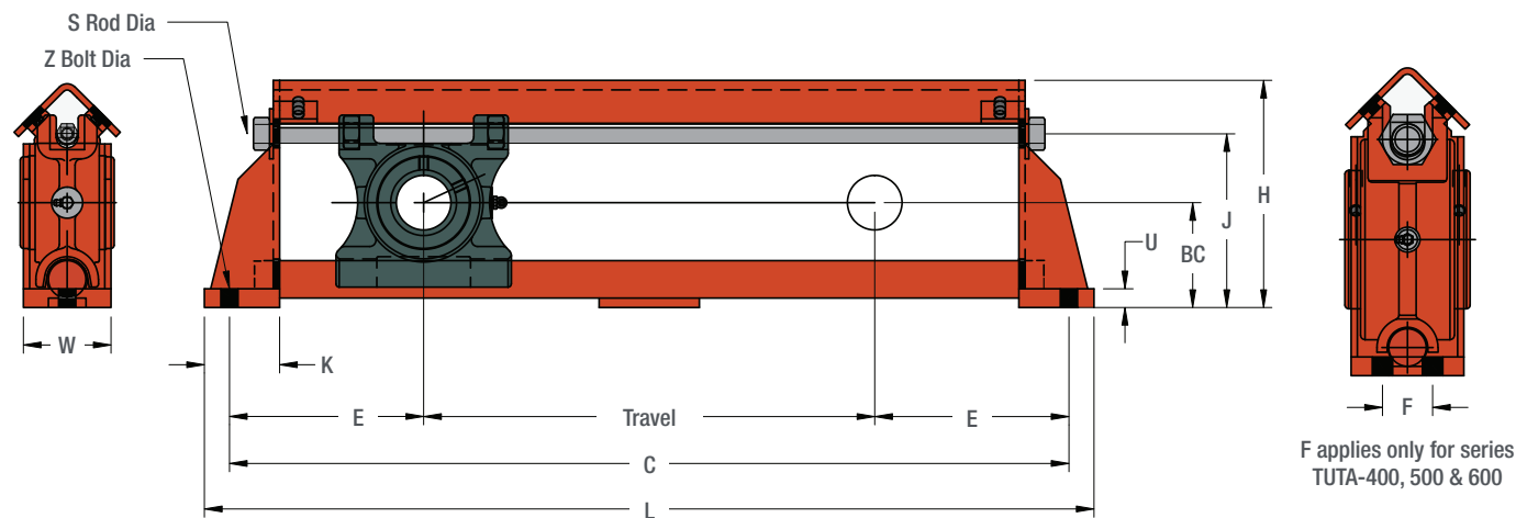
Figure 4.5 TUTA Drawings
