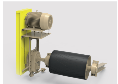
SHAFT MOUNT DRIVE ASSEMBLY
