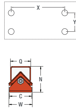
Figure 4.4-A TUHD Bearing bolt pattern EX.
