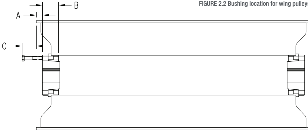
FIGURE 2.2 Bushing location for wing pulleys
