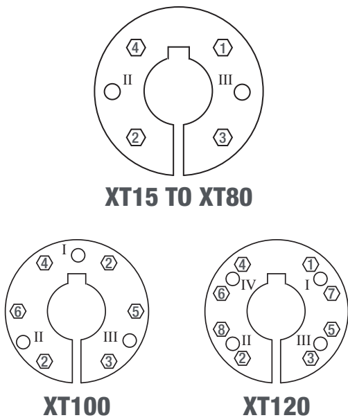
Figure 5.1 Numbered Capscrew Sequence
