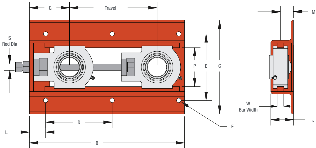
Figure 4.2 TUWS Drawings
